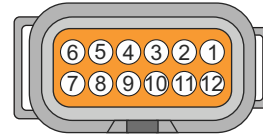
Wire side view of injector breakout connector
