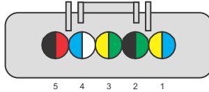
PLUG VIEW (WIRE SIDE) DENSO 197400-2090 (BASED ON SUBARU 2005 ADM WRX)
