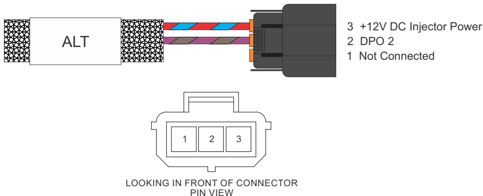
Figure 9 - Alternator Control Connection
