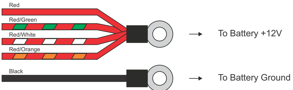
Figure 1 - Main Power Connections
