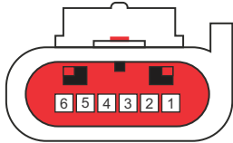
LOOKING INTO FRONT OF CONNECTOR (PIN VIEW)
