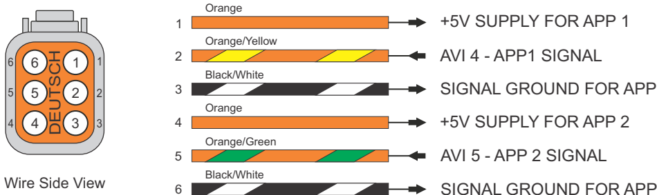
Figure 13 - Accelerator Pedal Position Harness Breakout Wiring
