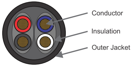
Cable Cross-Section
