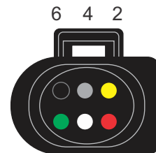
LSU4.9 connector Wire side view
